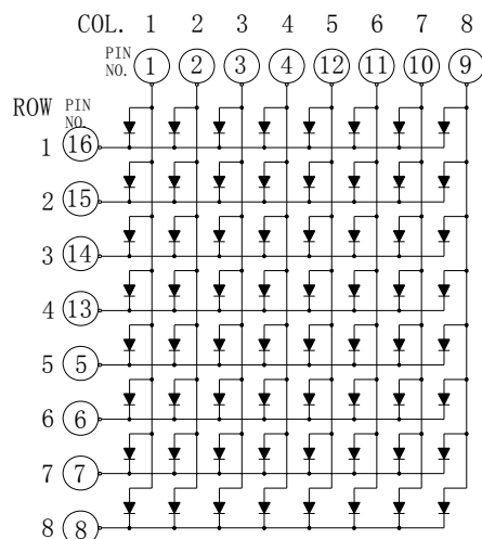
KWM-R30882CVB
