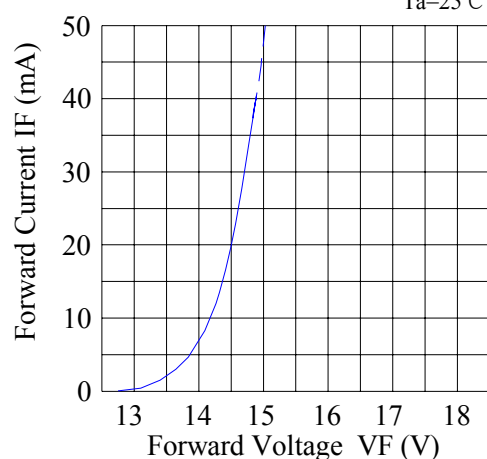
Forward Current & Forward Voltage Ta=25°C
