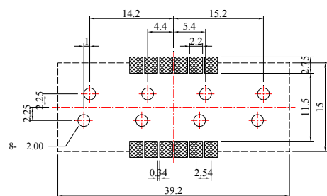
Recommended Soldering Pad Dimensions
