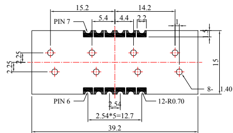
Recommended Soldering Pad Dimensions
