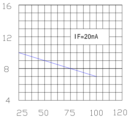
Fig.7 Relative Intensity vs. Ambient Temperature( )
