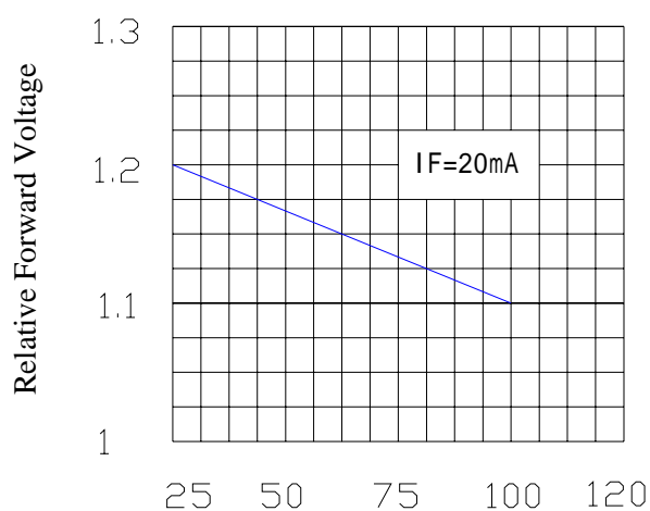
Fig.8 Forward Voltage vs. Ambient Temperature( )
