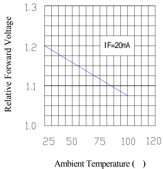
Fig.8 Forward Voltage vs. Ambient Temperature( )
