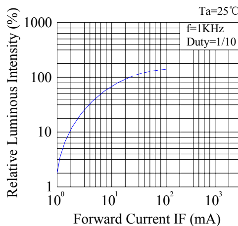
Luminous Intensity & Forward Current Ta=25°C
