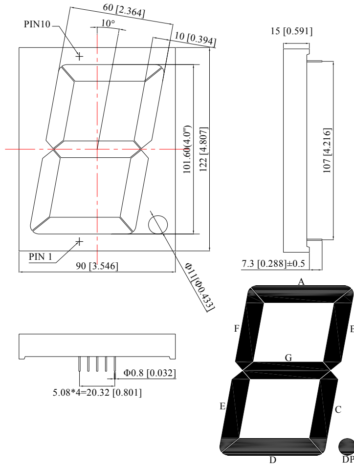
KW1-4001APGB
