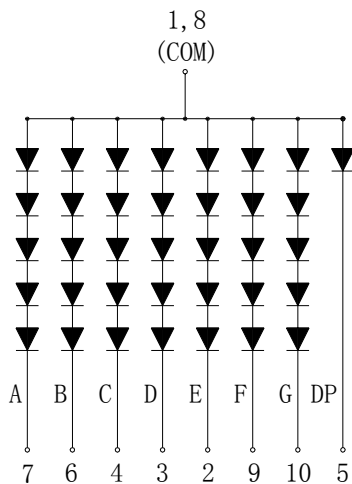
KW1-4001APGB
